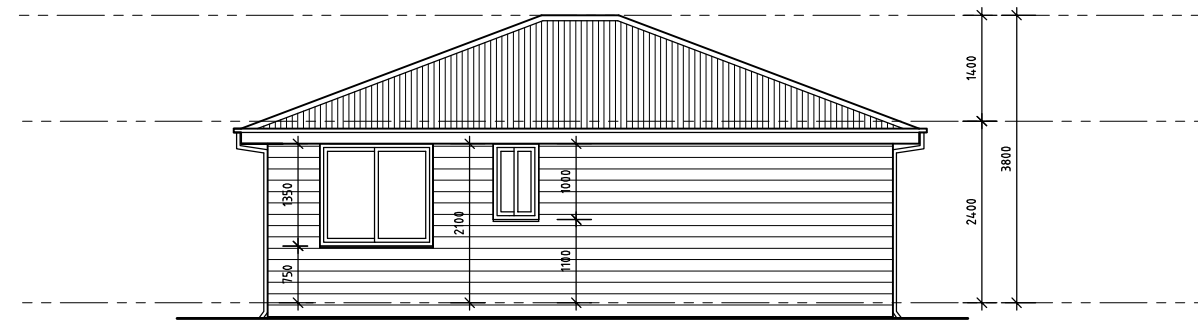
E REAR ELEVATION - 1:50
