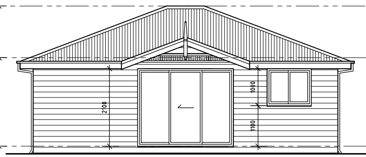
C FRONT ELEVATION - 1:50
