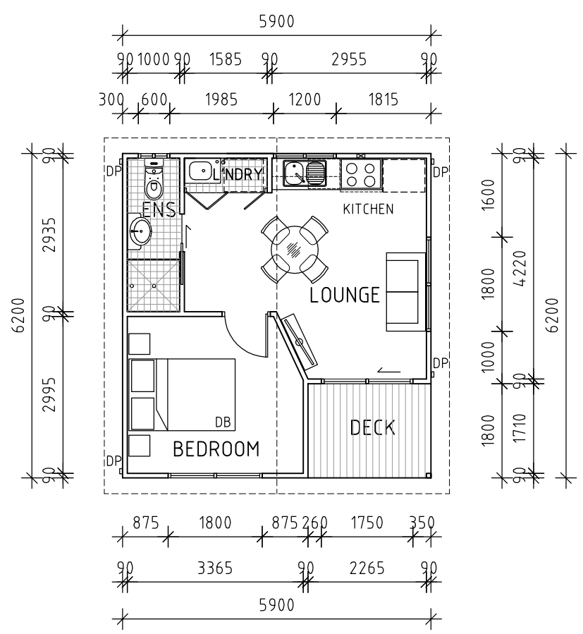
A 1 BED GRANNY FLAT FLOOR PLAN - 1:50
