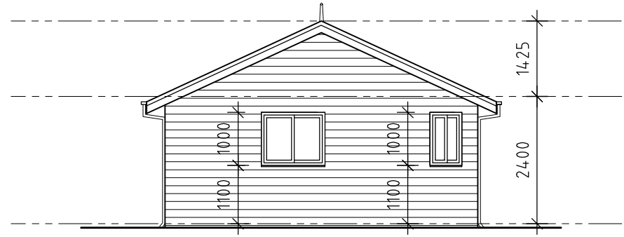
E REAR ELEVATION - 1:50
