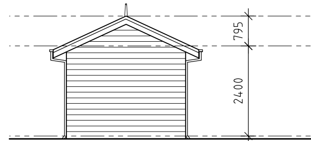
E REAR ELEVATION - 1:50
