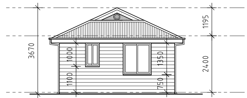
E REAR ELEVATION - 1:50
