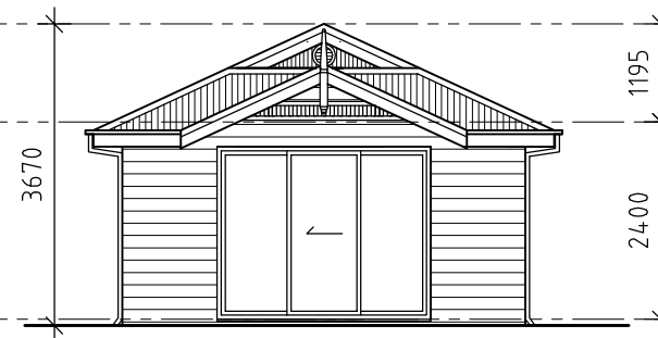
C FRONT ELEVATION - 1:50
