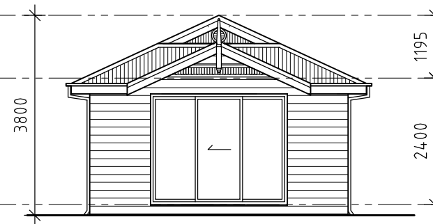
C FRONT ELEVATION - 1:50
